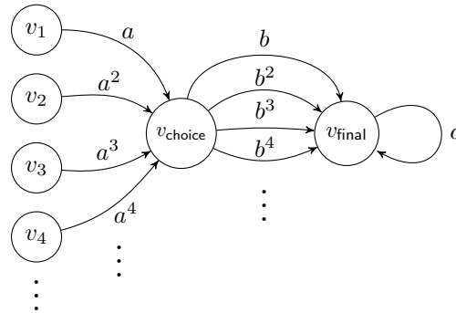
■ Figure 20 Outbidding game. First, a sequence a^n is produced, for some n \in \mathbb{N} . In order to win, Eve needs to answer with b^m , with m > n . Therefore, she can win from any vertex in the game, but no positional strategy guarantees the victory from all states.
