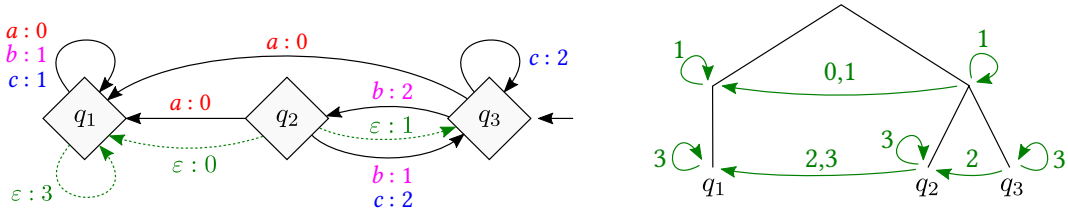
■ Figure 4 On the left, a deterministic automaton recognising the half-positional language \text{Inf}(a) \vee (\text{No}(a) \wedge \text{Fin}(bb)) . On the right, a representation of an \varepsilon -completion of the automaton. All arrows on the right correspond to \varepsilon -transitions that may be added without augmenting the language, such as the three dashed ones.
