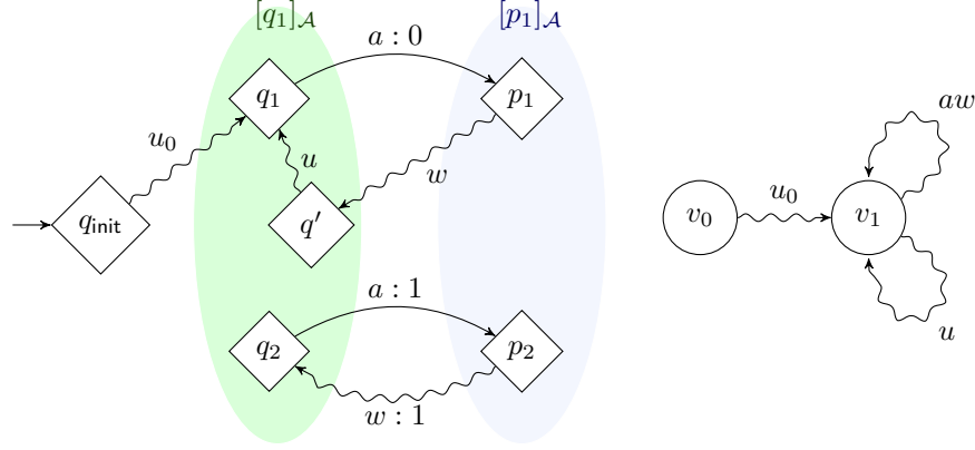
■ Figure 10 On the left, the situation in the automaton \mathcal{A} . We have the equivalences q_1 \sim_{\mathcal{A}} q_2 \sim_{\mathcal{A}} q' and p_1 \sim_{\mathcal{A}} p_2 . On the right, a game where Eve can win but not positionally.
