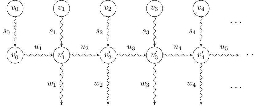
■ Figure 22 Game in which Eve wins if she produces a non-strictly increasing sequence of numbers. She can win from every v_i , but not positionally.
