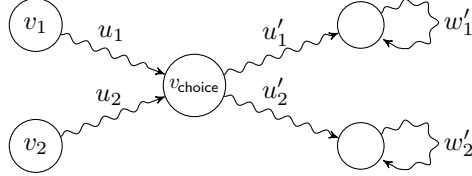
■ Figure 25 A game \mathcal{G} in which Eve cannot play optimally using positional strategies if \text{Res}(W) is not totally ordered.
