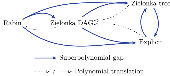
Figure 3 Comparison between the different representations of Muller conditions. A blue bold arrow from X to Y means that converting an X -representation into the form Y cannot be done in polynomial time. A dashed arrow from X to Y means the opposite. The dotted arrow indicates that the polynomial translation can only be applied on a fragment of X , as it is more expressive than Y .
