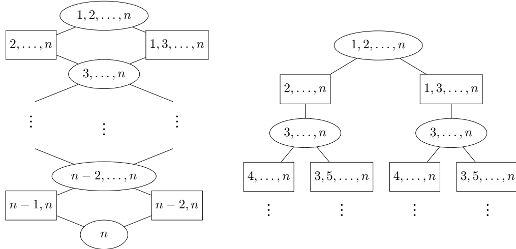
■ Figure 5 On the left, the Zielonka DAG of the condition \text{MinOddAndSucc}_n (for n odd), of size \mathcal{O}(n) . On the right, its Zielonka tree, of exponential size.
