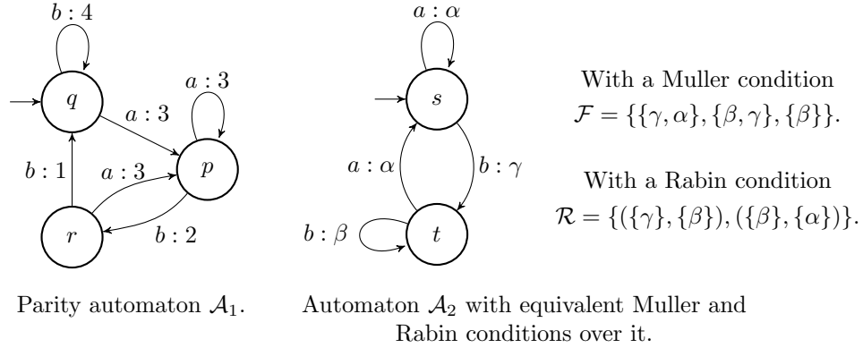
■ Figure 1 Different types of automata recognising the language L = \Sigma^* b^\omega + \Sigma^* (a^+ b)^\omega = \{w \in \Sigma^\omega \mid w \text{ has infinitely many } bs \text{ and finitely many } abb \text{ factors}\} . (Note that \{\beta, \gamma\} cannot result as the set of outputs occurring infinitely often in a run of \mathcal{A}_2 .)
