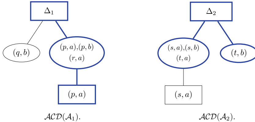
■ Figure 4 Alternating cycle decomposition of \mathcal{A}_1 and \mathcal{A}_2 , from Figure 1. In bold blue, the local subtrees of \mathcal{ACD}(\mathcal{A}_1) at p and of \mathcal{ACD}(\mathcal{A}_2) at t .
