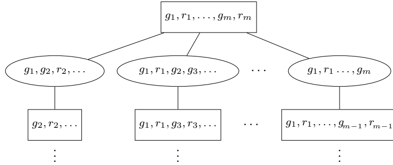
■ Figure 6 The Zielonka tree \mathcal{Z}_{\mathcal{F}_R} of the Rabin language from the proof of Proposition 5.9.
