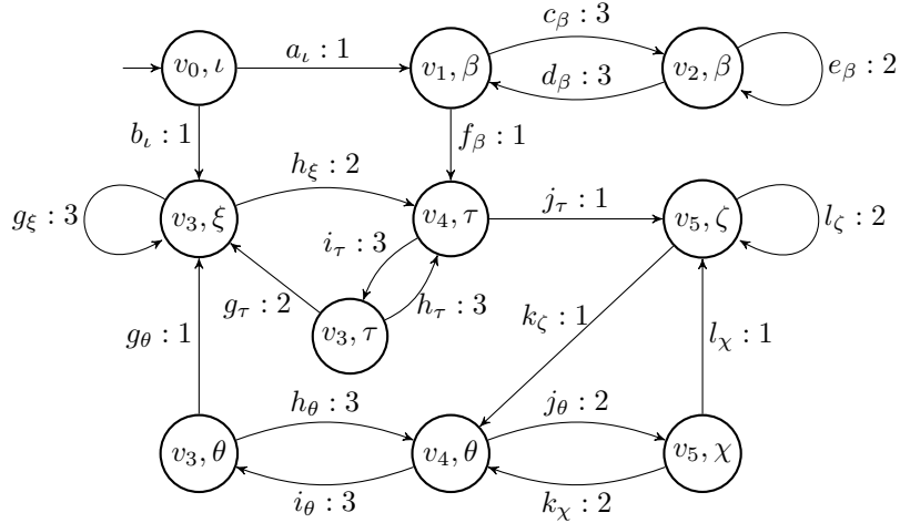
■ Figure 16 ACD-parity-transform \text{ACD}_{\text{parity}}(\mathcal{T}\mathcal{S}) of the transition system \mathcal{T}\mathcal{S} from Figure 14.
