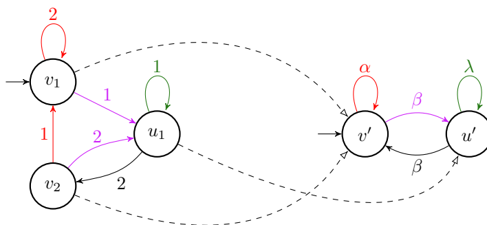
■ Figure 5 A locally bijective morphism from a parity TS to a Muller TS with acceptance set given by \mathcal{F} = \{\{\alpha\}, \{\beta\}\} . We use dashed arrows to represent the images of vertices, and colours to represent the image of edges (that can be inferred from \varphi_V ).
