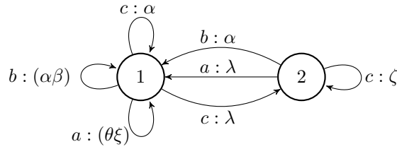
■ Figure 18 The simplified ZT-HD-Rabin-automaton.
