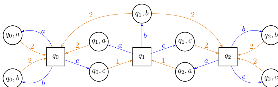
■ Figure 10 Letter game for the HD automaton from Figure 1, recognising the Muller language associated to \mathcal{F} = \{\{a\}, \{b\}, \{c\}, \{a, b\}, \{b, c\}\} . Squares represent Adam’s vertices (the states of the automaton) and circles Eve’s ones. Blue edges correspond to input-letters, and orange edges to the choices of transitions in the automaton after each input letter. The only vertex where Eve has a non-trivial choice to make to resolve the non-determinism of the automaton is (q_1, b) . In this example, Eve has a winning strategy corresponding to the resolver described in Example 2.3.
