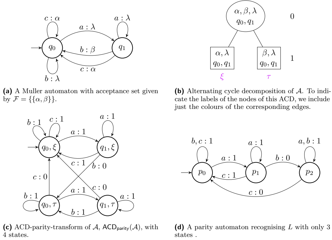
■ Figure 17 A minimal DMA whose ACD-parity-transform is not a minimal DPA.
