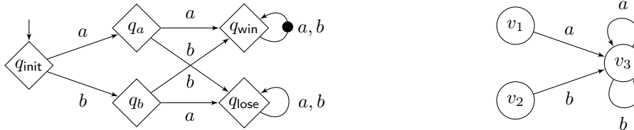
Figure 2: DBA \mathcal{B} recognizing objective W = (aa + bb)C^\omega (left), and an arena in which positional strategies do not suffice for \mathcal{P}_1 to play optimally for this objective (right). In figures, circles represent arena vertices controlled by \mathcal{P}_1 .
